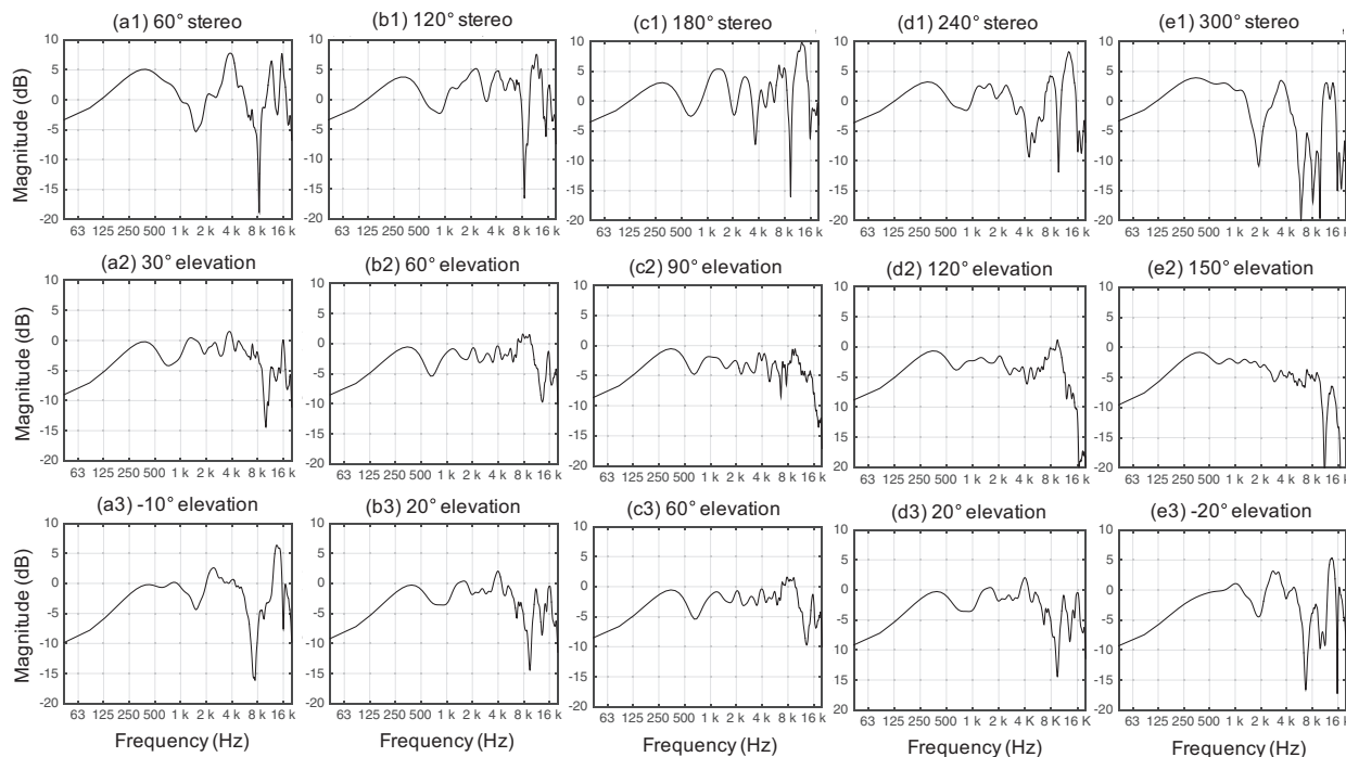
Fig. 9. The ear-input frequency spectra of phantom and real source signals measured using the MIT KEMAR dummy head database b . Each panel on the first row shows the spectrum of the left ear signal of a phantom center source resulting from each of the five loudspeaker base angles tested. Each panel on the second row shows the spectrum of the left ear signal for a real single source elevated in the median plane at half the base angle presented in the same column. Each panel on the bottom row presents the ear-input spectrum for a median plane elevation that produces the same first notch frequency as the base angle of the same column.
